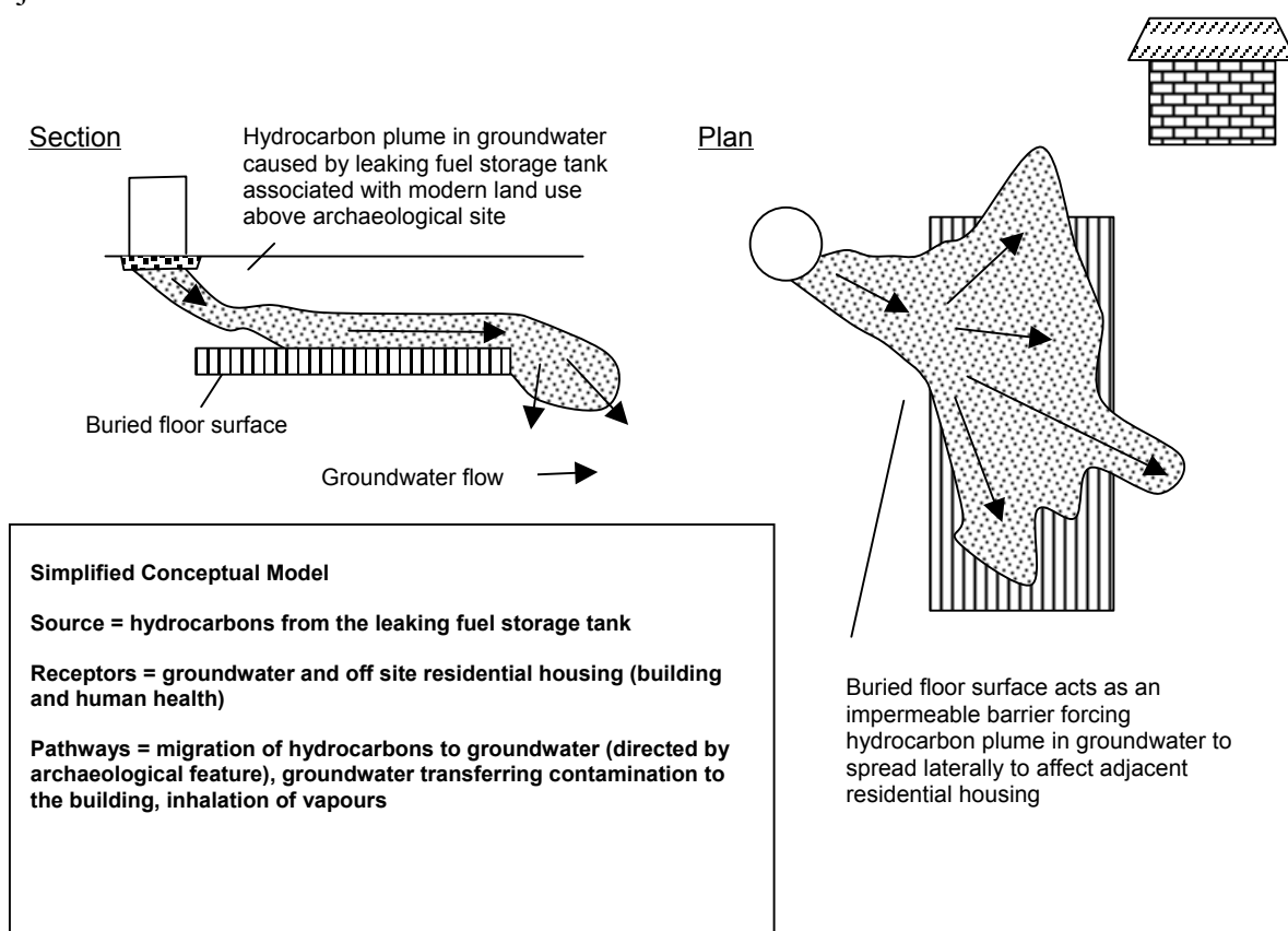
Figure 4.2 Archaeological feature acting as a barrier to the flow of contamination
